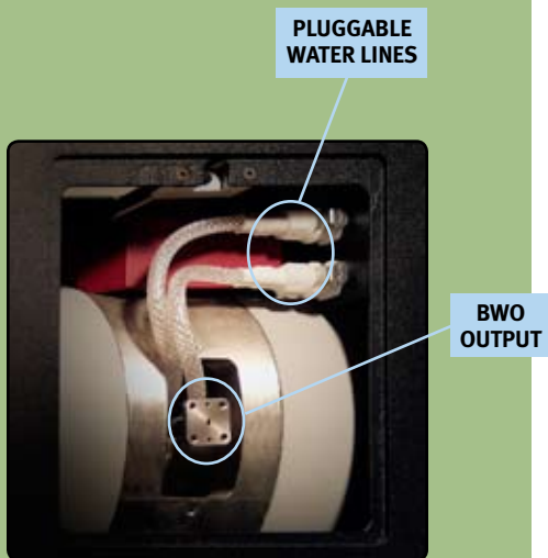
FRONT VIEW (OPEN FRONT PANEL)
