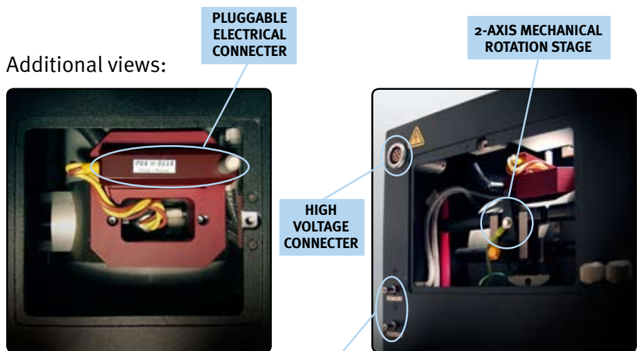
TOP VIEW (OPEN TOP PANEL)
